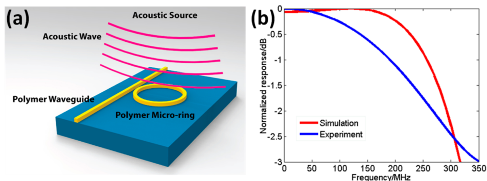
Figure 4. (a) Schematic drawing of the ring working as an acoustic resonator. (b) Simulated (red) and measured (blue) detector frequency response curves.
